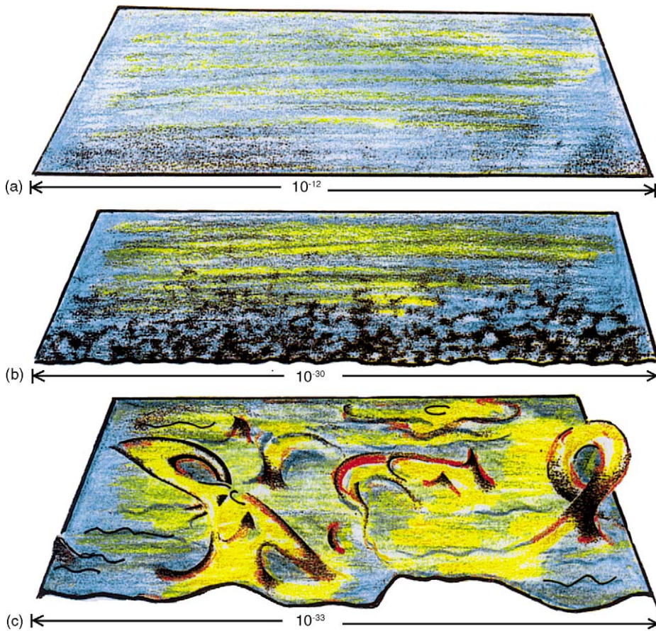
Fig. 2. A vision of the transformation of empty space from the smooth Euclidean to the rugged Planck-scale, after J.A. Wheeler's space–time foam (colouring by Sonya and Shareen El Naschie). The idea of introducing a universal length denoting the limit of measurement resolution is due to A. March (1936). W. Heisenberg attempted to abandon continuity ( \sim 1938 ) and used the classical radius of the electron as the smallest length L = 10^{-13} cm. A. Wheeler showed that general relativity and the uncertainty principle requires the topology and the dimensionality of space–time to fluctuate violently at the Planck length L_p = \sqrt{Gh/C^3} \cong 1.61 \times 10^{-33} . This L_p plays a significant role in modern physical theories such as strings.
