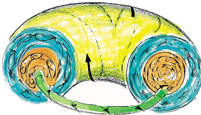
Fig. 1. A vague attractor of Kolmogorov (VAK), following Refs. [1,16]. Note that the fractal-like self-similarity of the VAK. VAK is also the goddess of vibration in the Rig-Veda which is most appropriate in the context of golden mean strings vibration.
