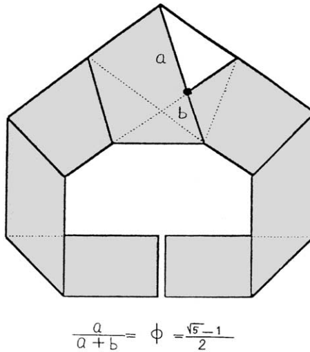
Fig. 5. An ordinary knot in a strip of paper produces a golden mean intersection of a perfect pentagon which is a part of a Möbius sling when ends are joined as indicated and the knot is made tight and carefully flattened. The corresponding theoretical knot is the well-known trefoil knot for which the hyperbolic volume is characteristically zero. Note that in the figure 8 knot possesses a hyperbolic volume equal to V_H = 2.02988321 \simeq \langle n \rangle = 2.078086921 . This may correspond to 't Hooft monopole solution of Yang–Mills–Higgs equation.
