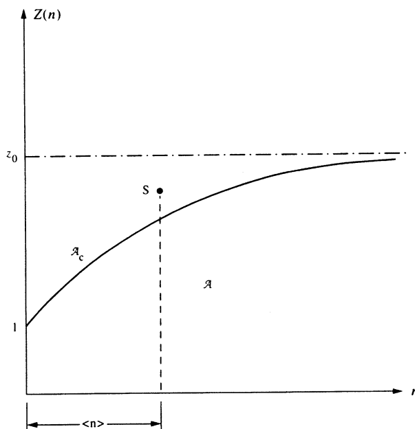
Fig. 6. Gamma space graphical interpretation of the expectation E(n) = \langle n \rangle of n as the coordinate \langle n \rangle = 2/\ln(1/d_c^{(0)}) of the centre of gravity S of the complementary area A_c above the curve z(n) which together with A forms an infinite rectangular space. In the discrete case, the curve becomes a polygon, z(n) becomes z_n = \sum_0^n (d_c^{(0)})^n , z_0 = \sum_0^\infty (d_c^{(0)})^n and \langle n \rangle = 2/\ln(1/d_c) becomes \sim \langle n \rangle = (1 + d_c^{(0)})/(1 - d_c^{(0)}) . The space z(n) is called the gamma space \Gamma(n, z_n) and details of the analysis can be found in [7,8].
