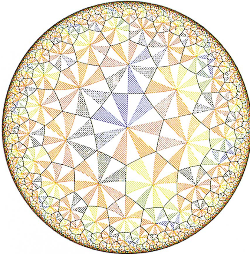
Fig. 4. A hyperbolic tiling in a Beltrami–Poincaré disk. The symmetries are those dictated by Möbius transformation in this case SL(2, \mathbb{R}) and one can clearly see Klein’s original modular curve inside the disk. From an intrinsically hyperbolic viewpoint, all triangles in the disk are identical. This is indirectly related to the existence of a scaling which is called the hyperbolic distance d . Note that the expectation of the normal distribution of the state of the Fischer transformation is half the value of the hyperbolic distance [32]. E(s) = 1/2(\ln(1 + \rho)/(1 - \rho))|_{r=\rho=\phi^3} = 0.240605912 . That means 1/E(s) = \langle n \rangle = 4.15617384 . Furthermore, the inverse of the hyperbolic distance is very close to the isomorphic length of the Penrose- E^{(\infty)} universe: 1/d = (\ln(1 + r)/(1 - r))^{-1} = [\ln(1/\phi)]^{-1} = 2.078086921 \simeq \ell/\rho where \ell \leq ((4 + \phi^3)/2)\rho = (2.118033989)(\rho) \simeq (2.078086921)(\rho) \cong 1/d . Another note worthy fact is that the constituent mass of the light quarks m_u^* \simeq m_d^* \simeq 336 MeV is related to the number of triangles of Klein’s original curve namely n = (2)(168) = 336 . This geometry corresponds to the internal geometry of Nonabelian gauge groups.
