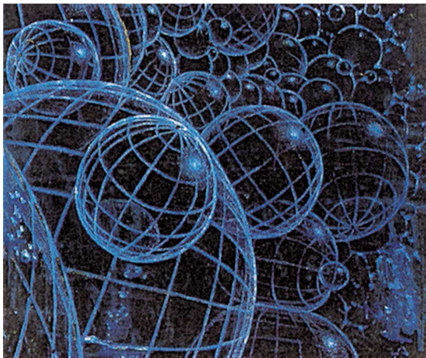
Fig. 3. Turbulent Appollonian spheres on all scales as a model for e^{(\infty)} space or a kind of polymerized spherical micro-space–time. This is just an artistic impression and should not be taken literally.
